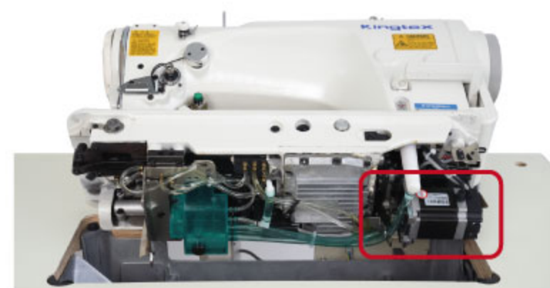
SR雙步進款 SR Double Stepping Motor Type
