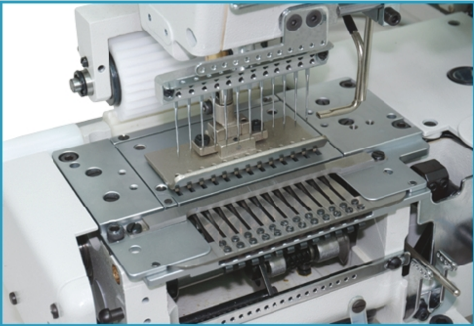
UT12A 切底線裝置 Under bed thread trimmer
