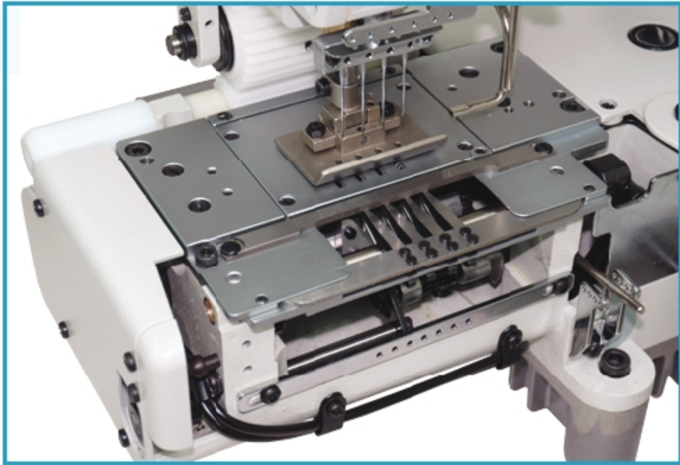
UT04A 切底線裝置 Under bed thread trimmer
