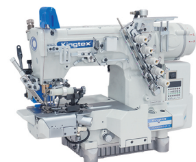
CXM2085-0-356M Attaching Pre-Closed Flat Knit Elastic Band Onto Waists Of Tubular Goods (With Right Knife, Rear Puller & Chips Suction Pipe)
