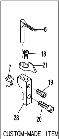
FOR MODEL MT4513-MT4517
